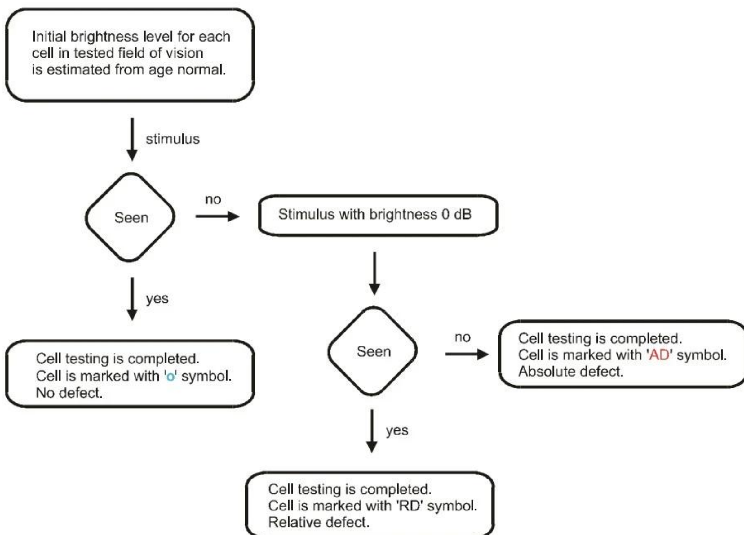
Pic. 51. 3 Zone strategy algorithm.
