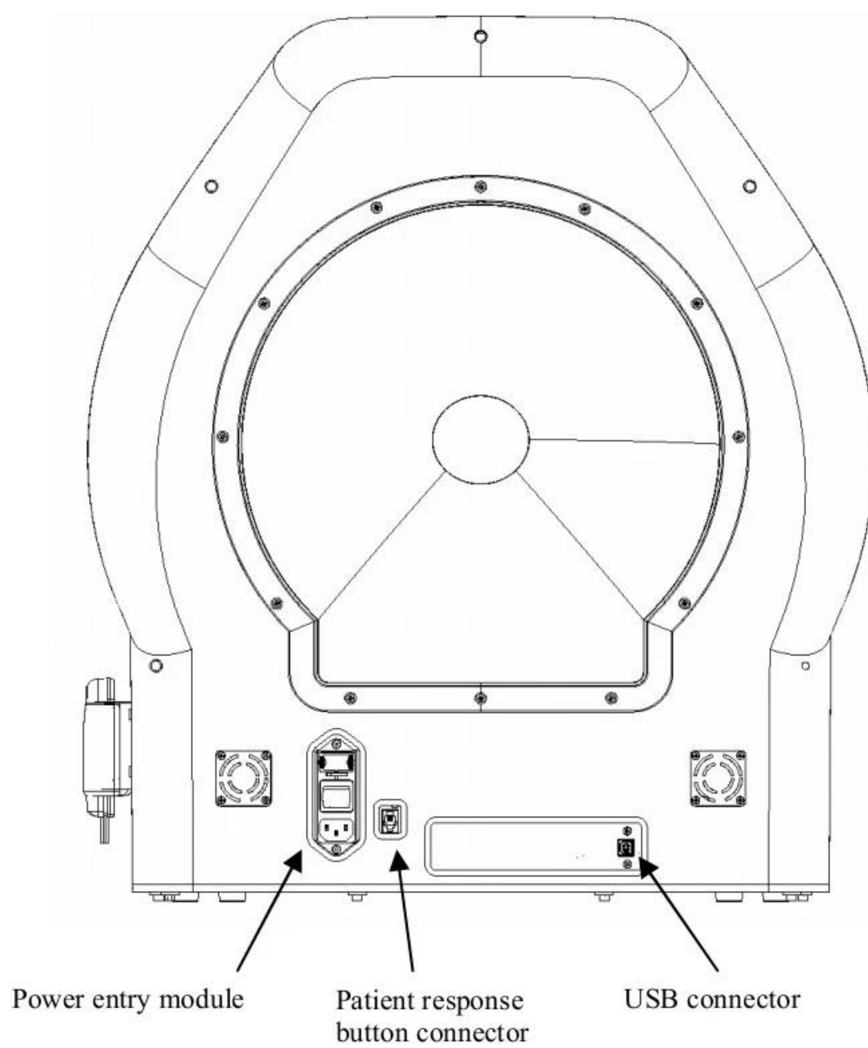
Rear view and connectors
