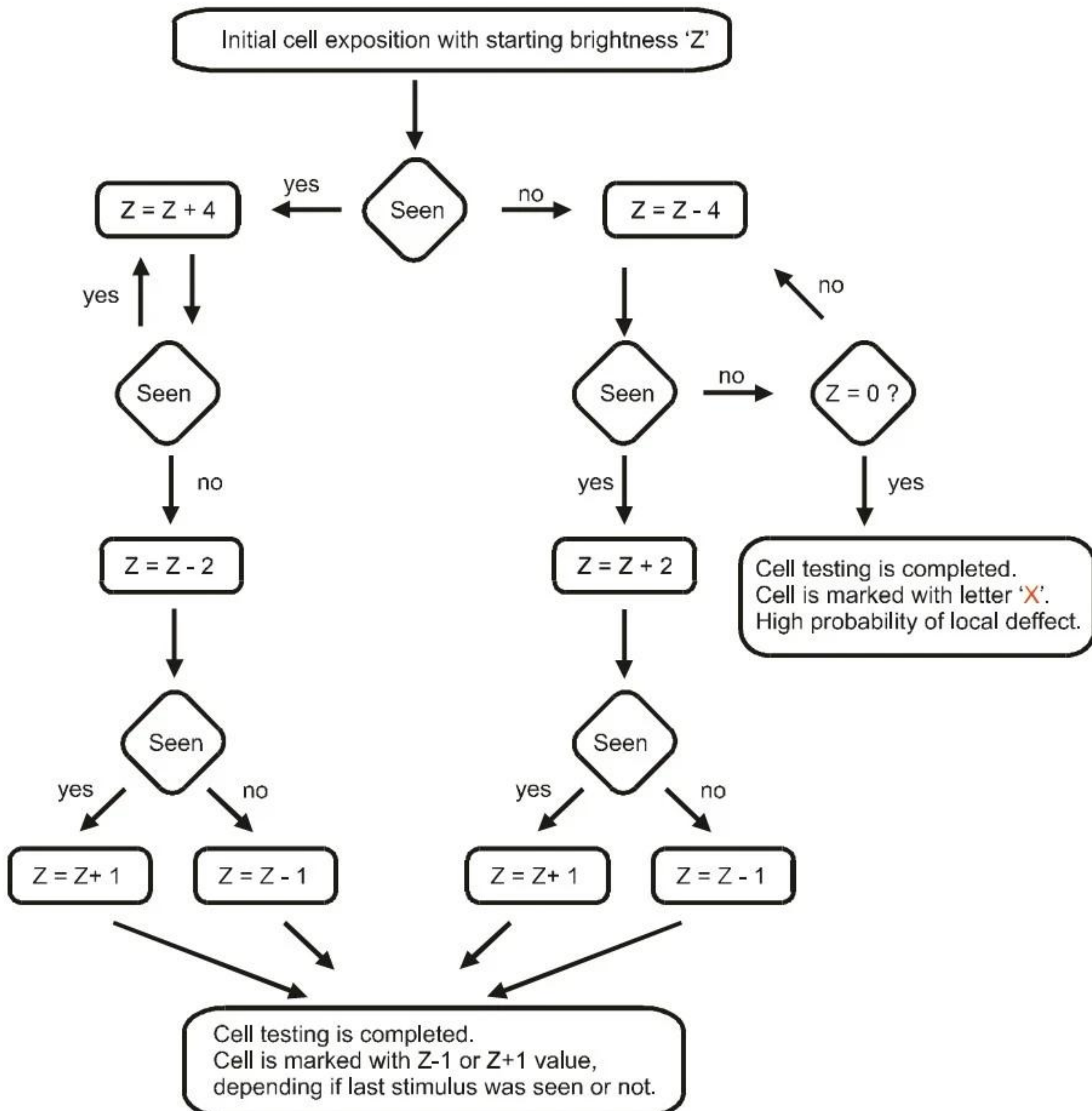
Pic. 53. Fast Threshold algorithm
